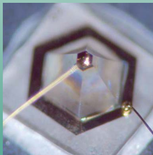
Mega-cone blue LEDs based on ZnO/GaN direct wafer bonding (A. Murai, D. B. Thompson, H. Masui, N. Fellows, U. K. Mishra, S. Nakamura, and S. P. DenBaars, p. 2756)
