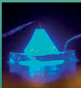
Mega-cone blue LEDs based on ZnO/GaN direct wafer bonding (A. Murai, D. B. Thompson, H. Masui, N. Fellows, U. K. Mishra, S. Nakamura, and S. P. DenBaars, p. 2756)
