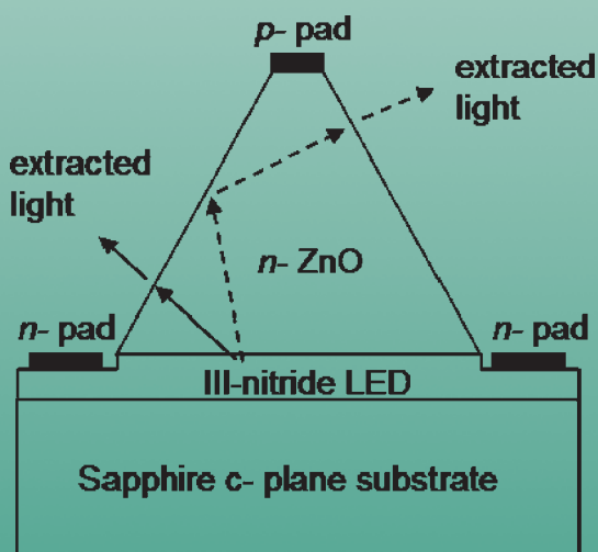
Mega-cone blue LEDs based on ZnO/GaN direct wafer bonding (A. Murai, D. B. Thompson, H. Masui, N. Fellows, U. K. Mishra, S. Nakamura, and S. P. DenBaars, p. 2756)
